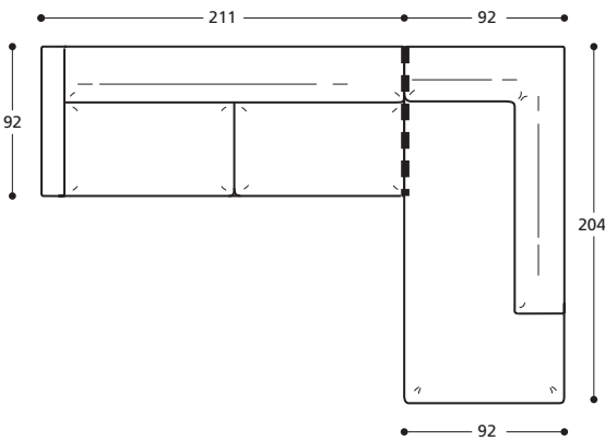
1 X Art. 1749 ELEMENT 211 1 X Art. 1752 SCHLUSSECKELEMENT 204
