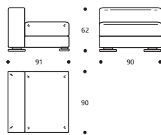
Art. 1868 91 X 90 X h. 62 cm
