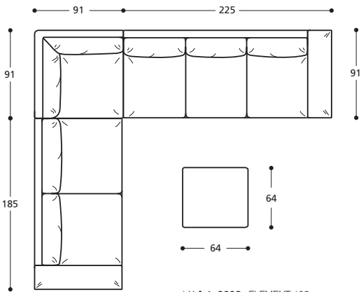
1 X Art. 9608 ELEMENT 185 1 X Art. 9619 CORNER 91X91 1 X Art. 9610 ELEMENT 225 1 X Art. 9614 POUF 64X64
